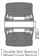
[Double Ball Bearing Wheel Cross Section]
