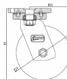
Plane Bearing Demonstration
