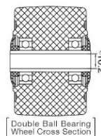
[Double Ball Bearing Wheel Cross Section]
